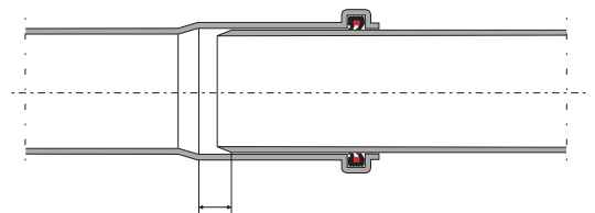
Dış Çap (mm) S1 (mm) S2 (mm) S3 (mm) LB Ağırlık (kg/m) 50 3.0 2.9 2.4 39.3 0.708 75 3.0 2.9 2.4 46.1 1.088 110 3.2 2.9 2.4 56.9 1.619 125 3.2 2.9 2.4 62.8 1.850 160 4.0 3.6 3.0 75.8 2.948 200 4.9 4.4 3.7 89.4 4.502 250 6.2 5.6 4.7 112.6 7.073 315 7.7 6.9 5.8 135.4 11.043
