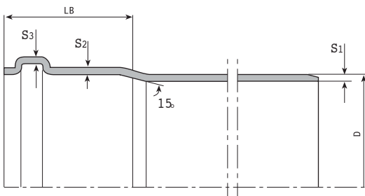
Dış Çap (mm) S1 (mm) S2 (mm) S3 (mm) LB Ağırlık (kg/m) 50 3.0 2.9 2.4 39.3 0.708 75 3.0 2.9 2.4 46.1 1.088 110 3.2 2.9 2.4 56.9 1.619 125 3.2 2.9 2.4 62.8 1.850 160 4.0 3.6 3.0 75.8 2.948 200 4.9 4.4 3.7 89.4 4.502 250 6.2 5.6 4.7 112.6 7.073 315 7.7 6.9 5.8 135.4 11.043
