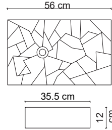
E-W2000 Tezgah Üstü Lavabo Over-the counter basin
