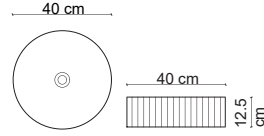
E-W1001MF Tezgah Üstü Lavabo Over-the counter basin
