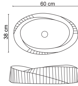
EY-4706 Tezgah Üstü Lavabo Over-the counter basin
