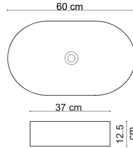
E-W1202MM Tezgah Üstü Lavabo Over-the counter basin
