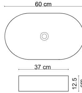
E-W1202MS Tezgah Üstü Lavabo Over-the counter basin
