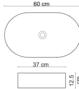
E-W1202 Tezgah Üstü Lavabo Over-the counter basin
