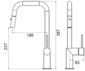
VM-2141 Vario Pull Out Kitchen Mixer - Chrome Eviye Bataryası - Krom
