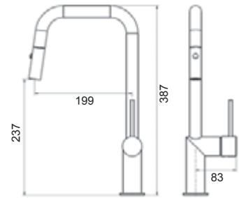
VM-2144 Vario Pull Out Kitchen Mixer - Brushed Gold Eviye Bataryası - Brushed Gold
